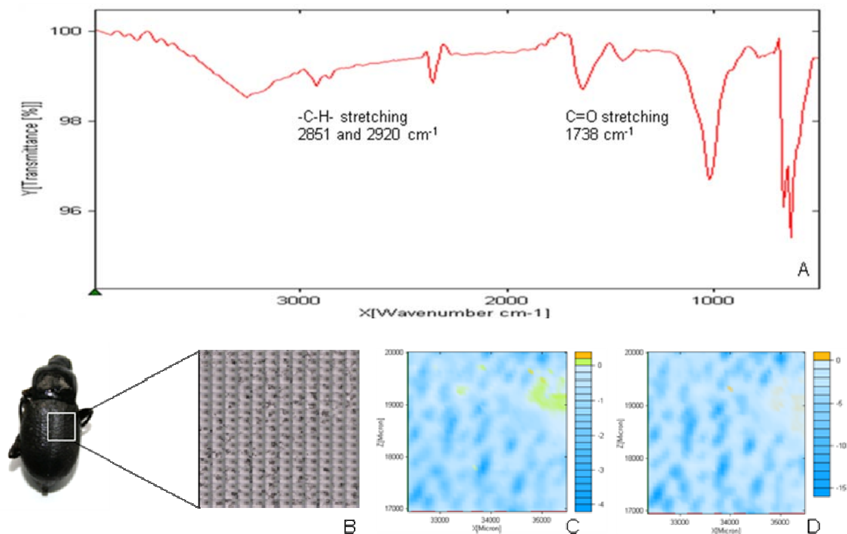
Fig. 4. IR imaging of B. femoralis surface lipids
